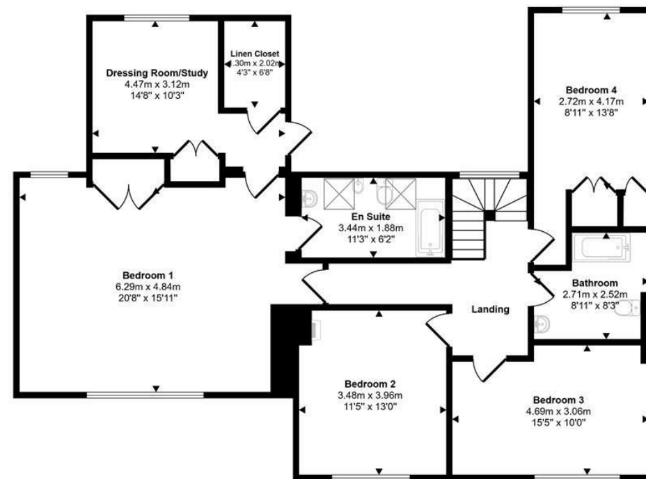
First Floor Approx 120 sq m / 1287 sq ft
