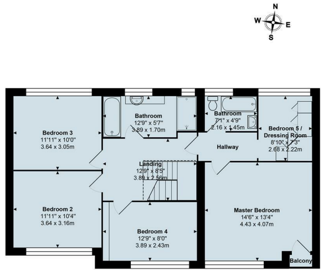
First Floor Area: 878 ft 2 ... 81.6 m 2
