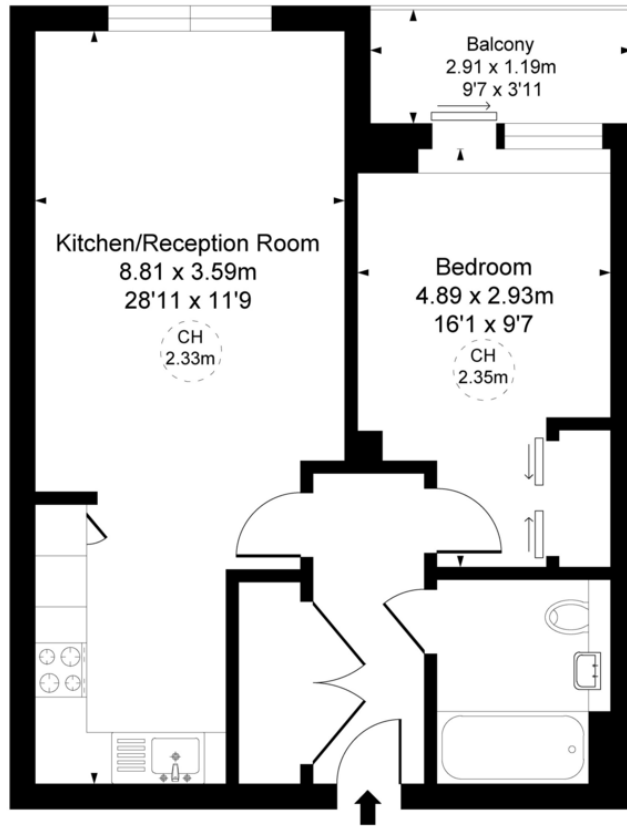
Sixth Floor
