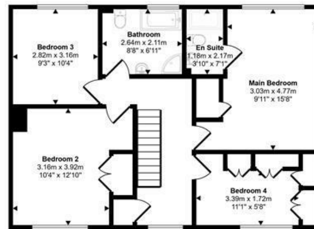
First Floor Approx 73 sq m / 790 sq ft
