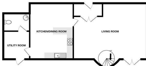
GROUND FLOOR
