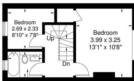
First Floor 29.3 sq m / 315 sq ft
