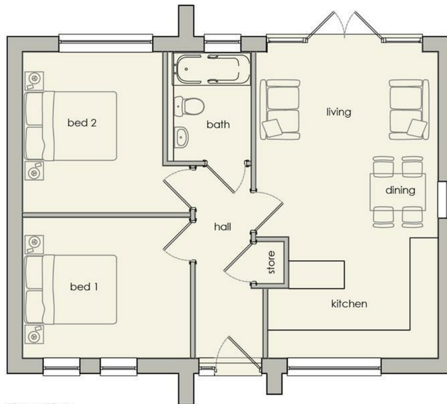
Floor Plan
