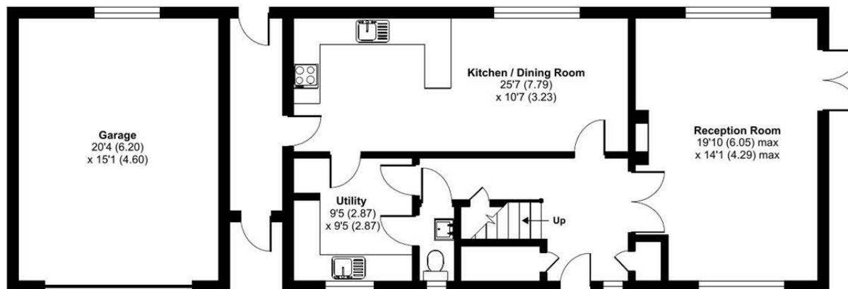
GROUND FLOOR
