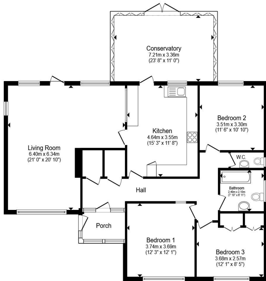
Floor Plan 1
