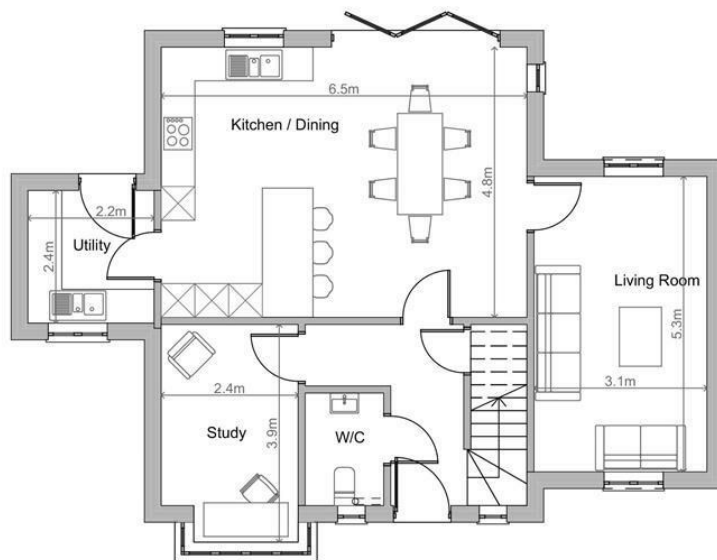
Ground Floor 1:100
