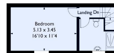
The Cottage First Floor
