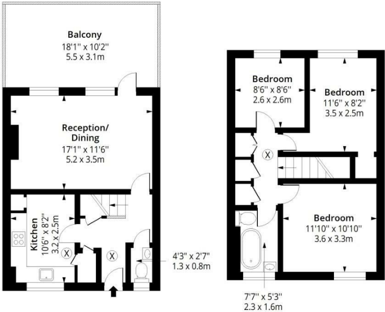
First Floor Floor Area 398 Sq Ft - 36.97 Sq M
