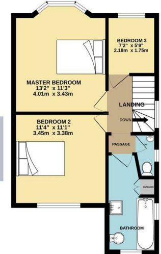
FIRST FLOOR 439 sq.ft. (40.3 sq.m.) approx.
