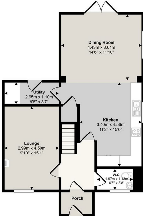
Ground Floor Approx 63 sq m / 679 sq ft
