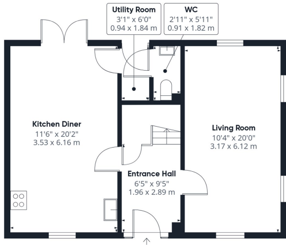
Floor 0 Building 1
