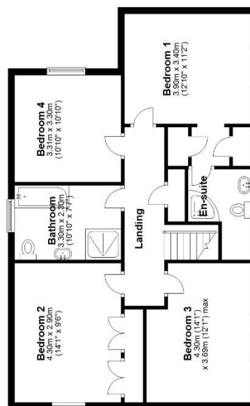
First Floor Approx. 79.9 sq. metres (859.3 sq. feet)
