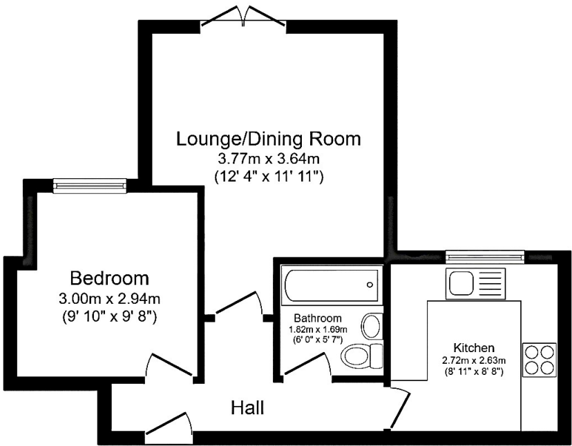
Floor Plan
