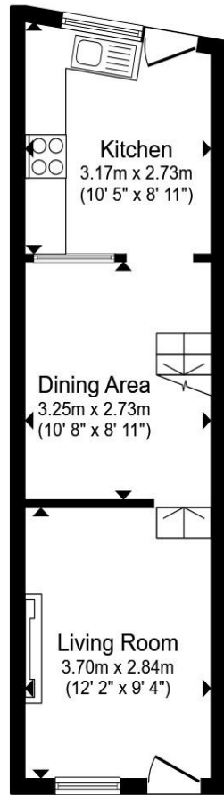
Ground Floor
