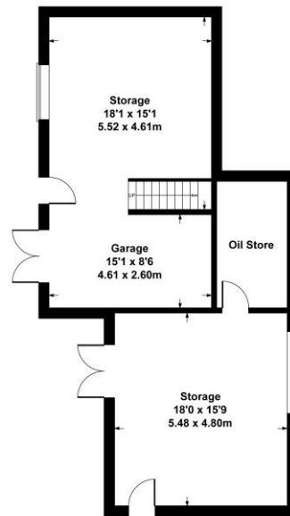
GROUND FLOOR OUTBUILDING
