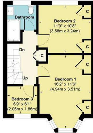
First Floor Approximate Floor Area 468 sq.ft (43.51 sq.m)
