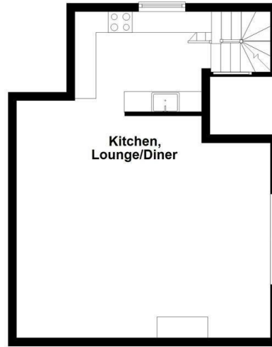
Top Floor
