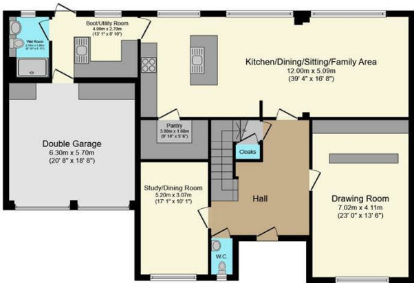
Ground Floor Floor area 122.5 sq.m. (1,318 sq.ft.)
