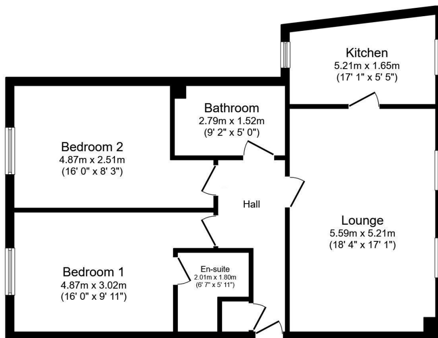
Floor Plan Floor area 71.7 sq.m. (772 sq.ft.)
