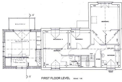
FIRST FLOOR LEVEL SCALE 1:50
