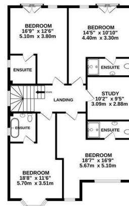
1ST FLOOR 1060 sq.ft. (98.5 sq.m.) approx.
