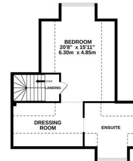
2ND FLOOR 606 sq.ft. (56.3 sq.m.) approx.
