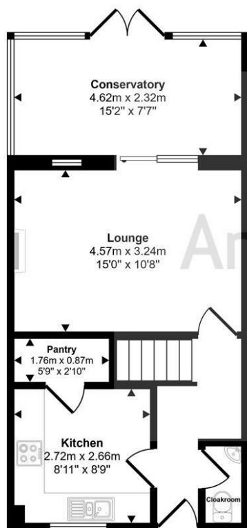
Ground Floor Approx 44 sq m / 478 sq ft
