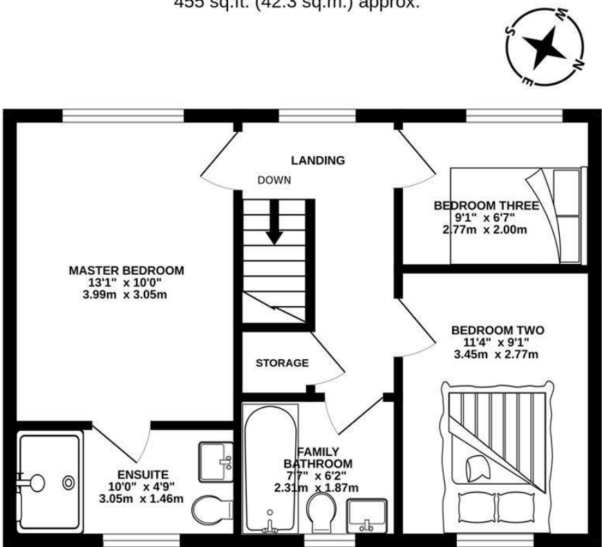
1ST FLOOR 455 sq.ft. (42.3 sq.m.) approx.
