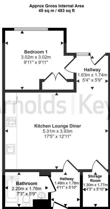
Floorplan
