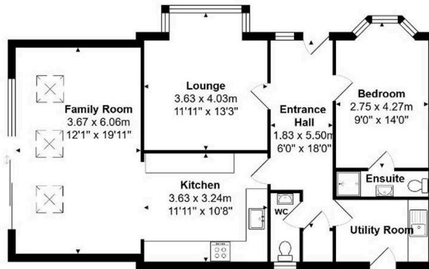
GROUND FLOOR Area: 79.6 m 2 ... 856 ft 2
