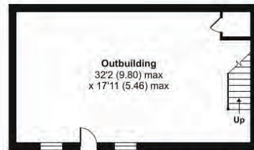
OUTBUILDING 1 GROUND FLOOR
