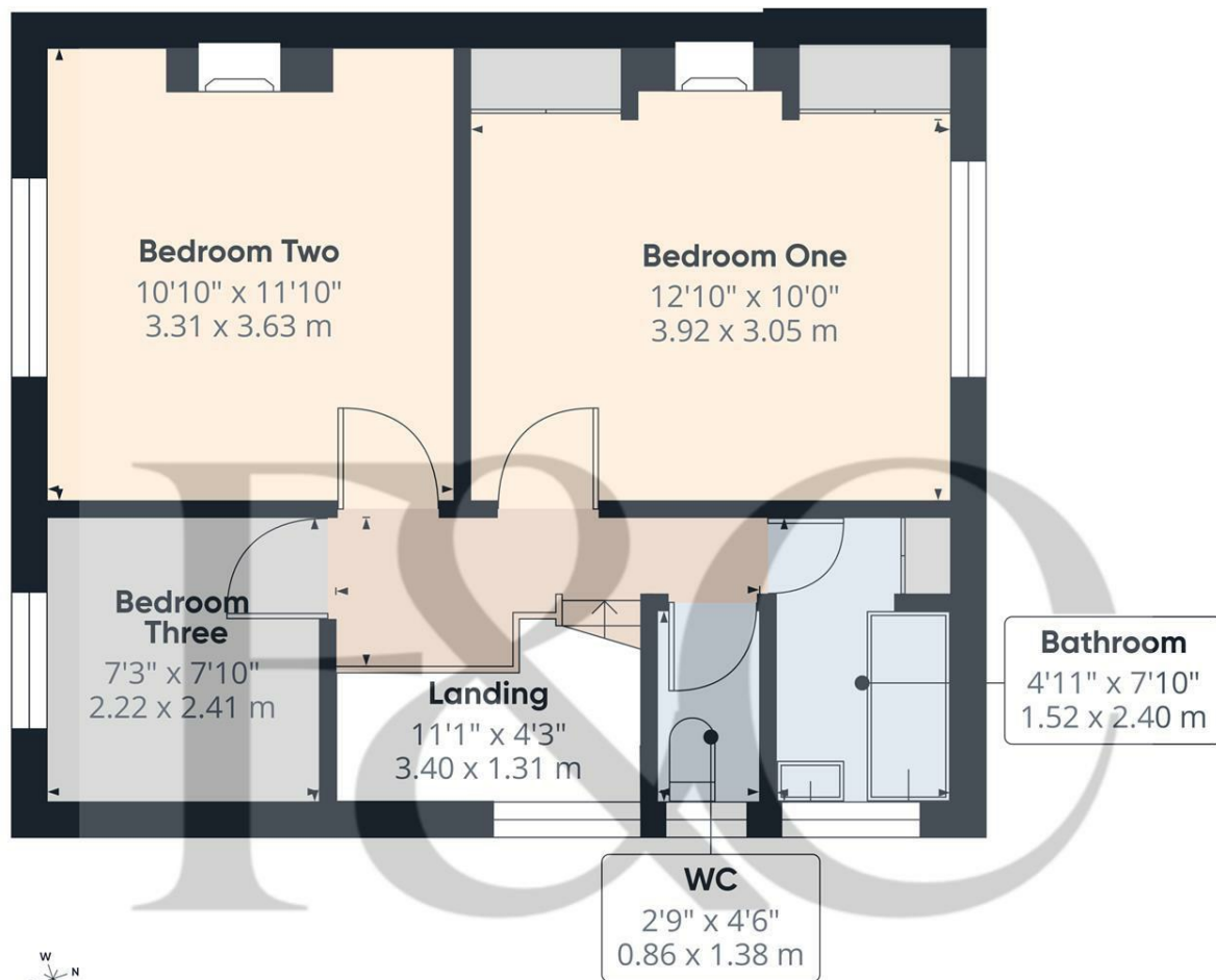
Floor 1
