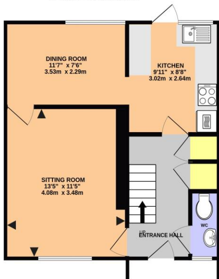
GROUND FLOOR 477 sq.ft. (44.3 sq.m.) approx.
