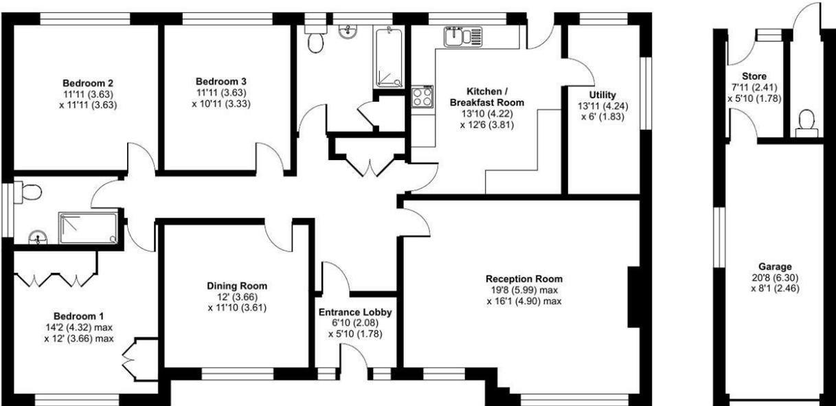
GROUND FLOOR
