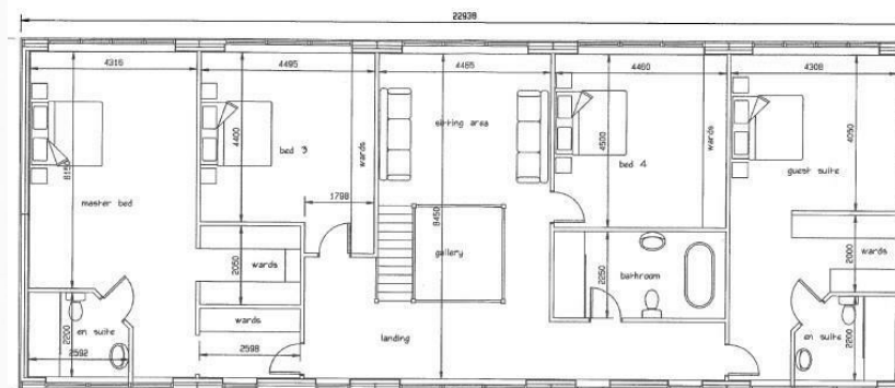
Proposed First Floor Plan 1:50
