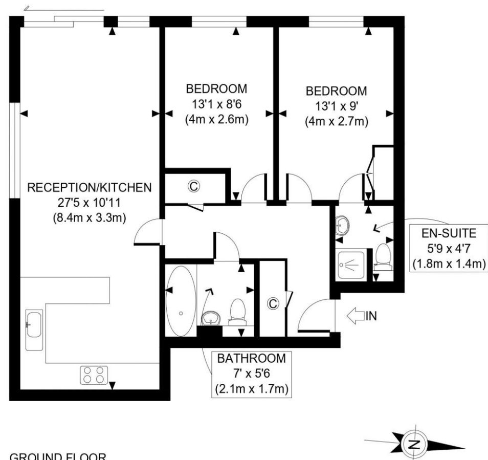
GROUND FLOOR GROSS INTERNAL FLOOR AREA 708 SQ FT
