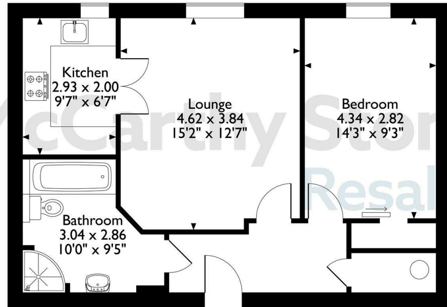
The position & size of doors, windows, appliances and other features are approximate only. © ehous. Unauthorised reproduction prohibited. Drawing ref. dig/8652859/DST.
