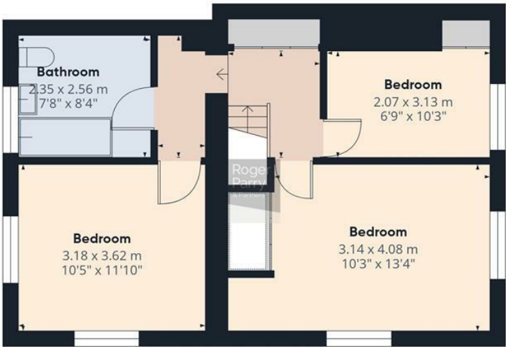
Floor 1 Building 1
