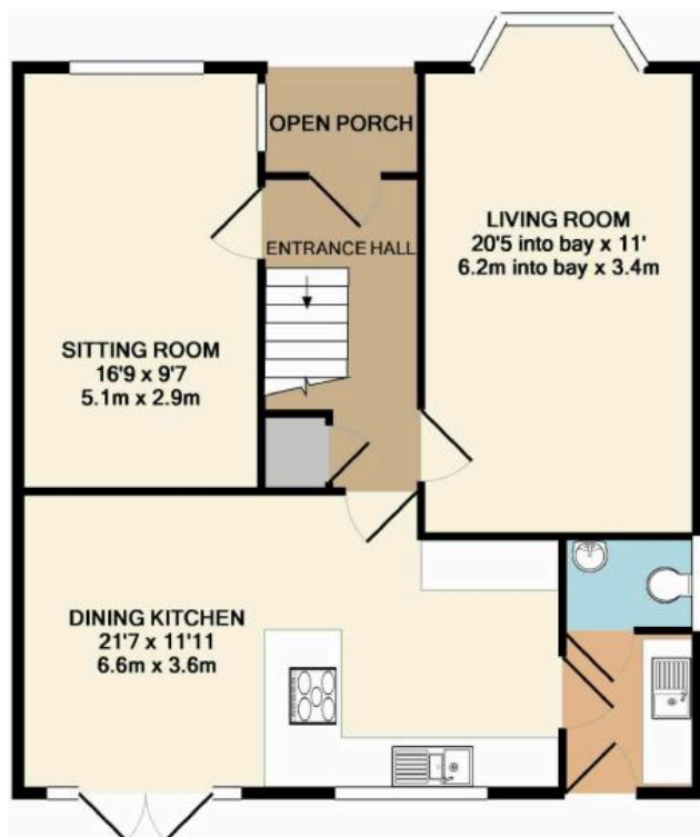
GROUND FLOOR APPROX. FLOOR AREA 786 SQ.FT. (73.0 SQ.M.)
