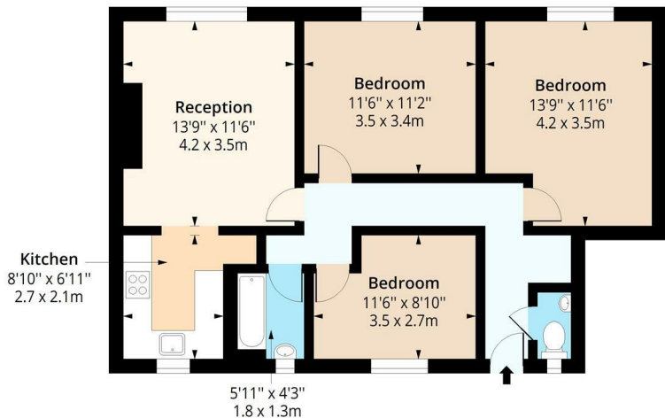
Ground Floor Floor Area 789 Sq Ft - 73.30 Sq M
