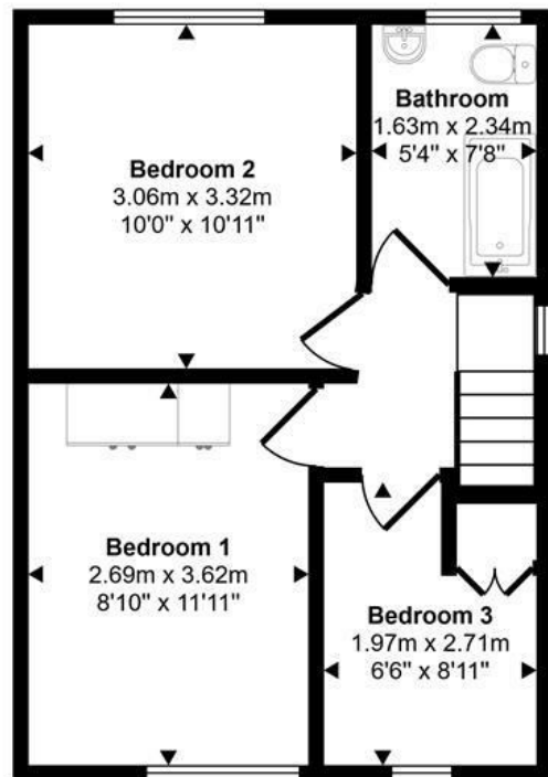
First Floor Approx 34 sq m / 367 sq ft
