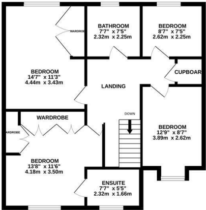
1ST FLOOR 726 sq.ft. (67.4 sq.m.) approx.
