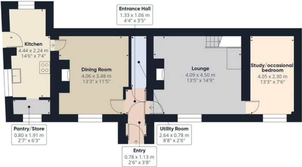
Floor 0 Building 1
