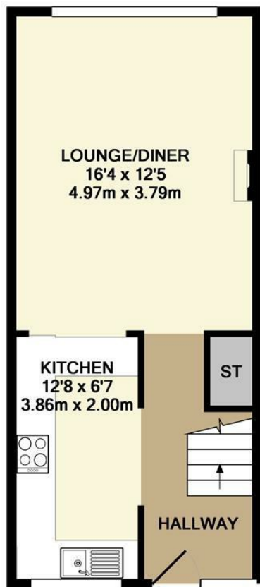
GROUND FLOOR APPROX. FLOOR AREA 360 SQ.FT. (33.5 SQ.M.)
