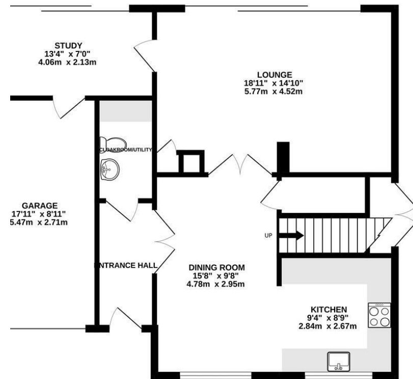
GROUND FLOOR 865 sq.ft. (80.4 sq.m.) approx.
