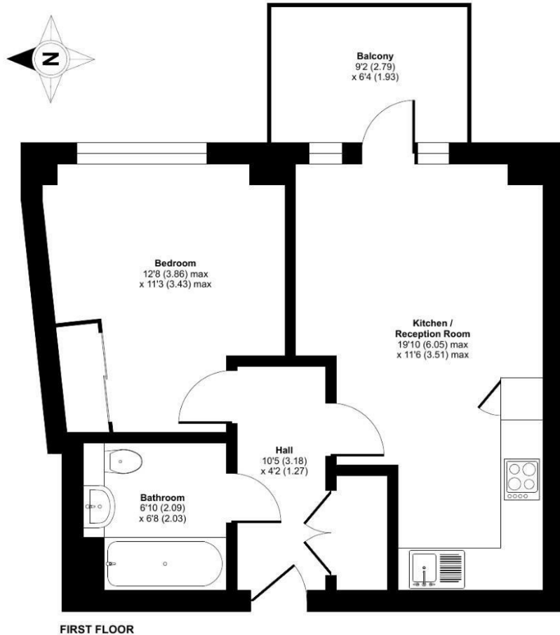
FIRST FLOOR
