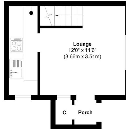
Ground Floor Approximate Floor Area 209 sq. ft (19.41 sq. m)
