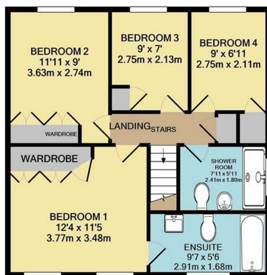
1ST FLOOR APPROX. FLOOR AREA 534 SQ.FT. (49.6 SQ.M.)
