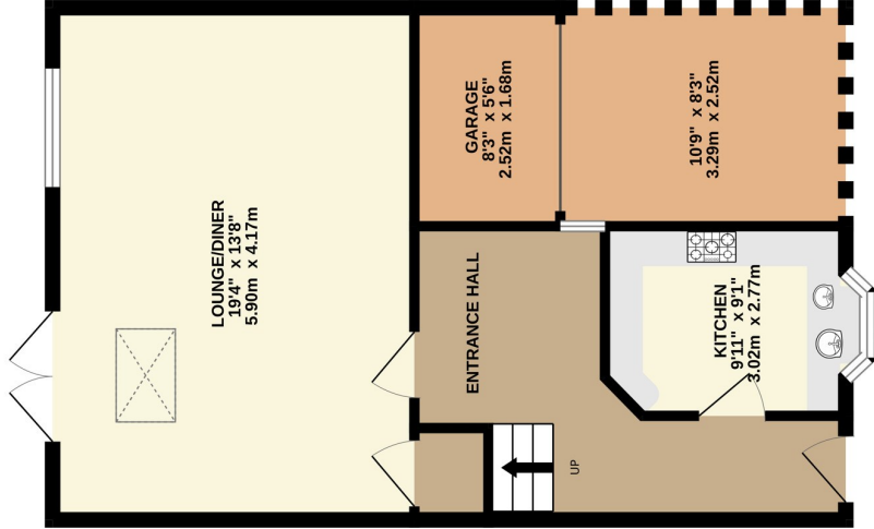
GROUND FLOOR 583 sq.ft. (54.2 sq.m.) approx.
