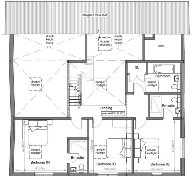
Proposed Mezzanine floor plan (Barn 01)
