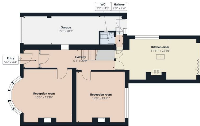
Floor 0
